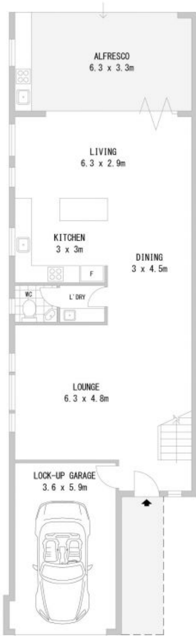
GROUND FLOOR
