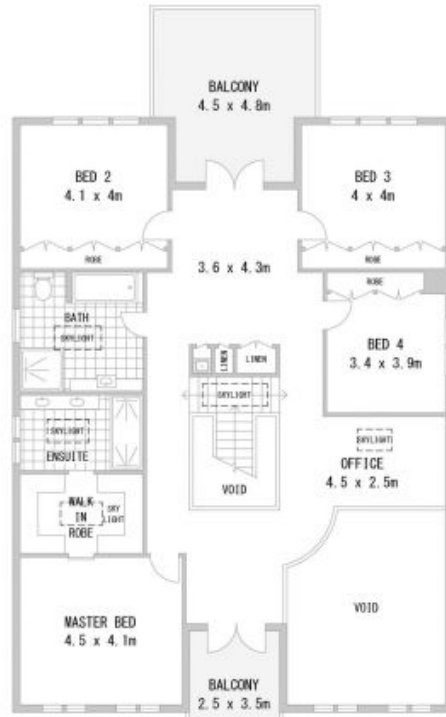
LEVEL ONE
