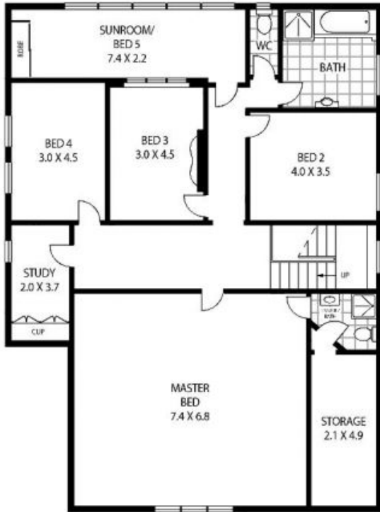
LEVEL ONE
