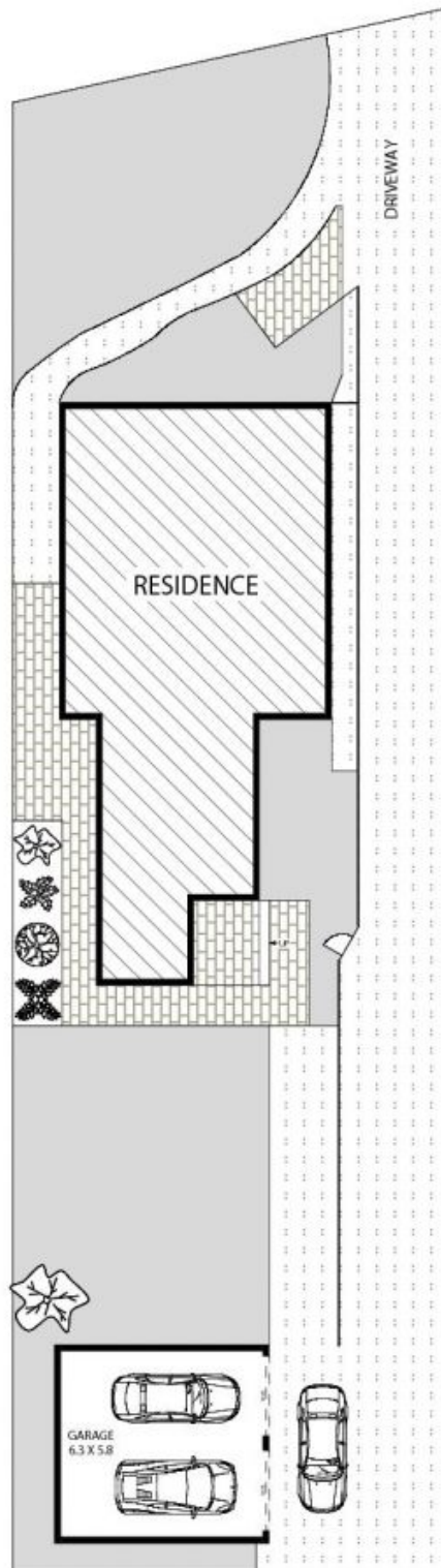
SITE PLAN
